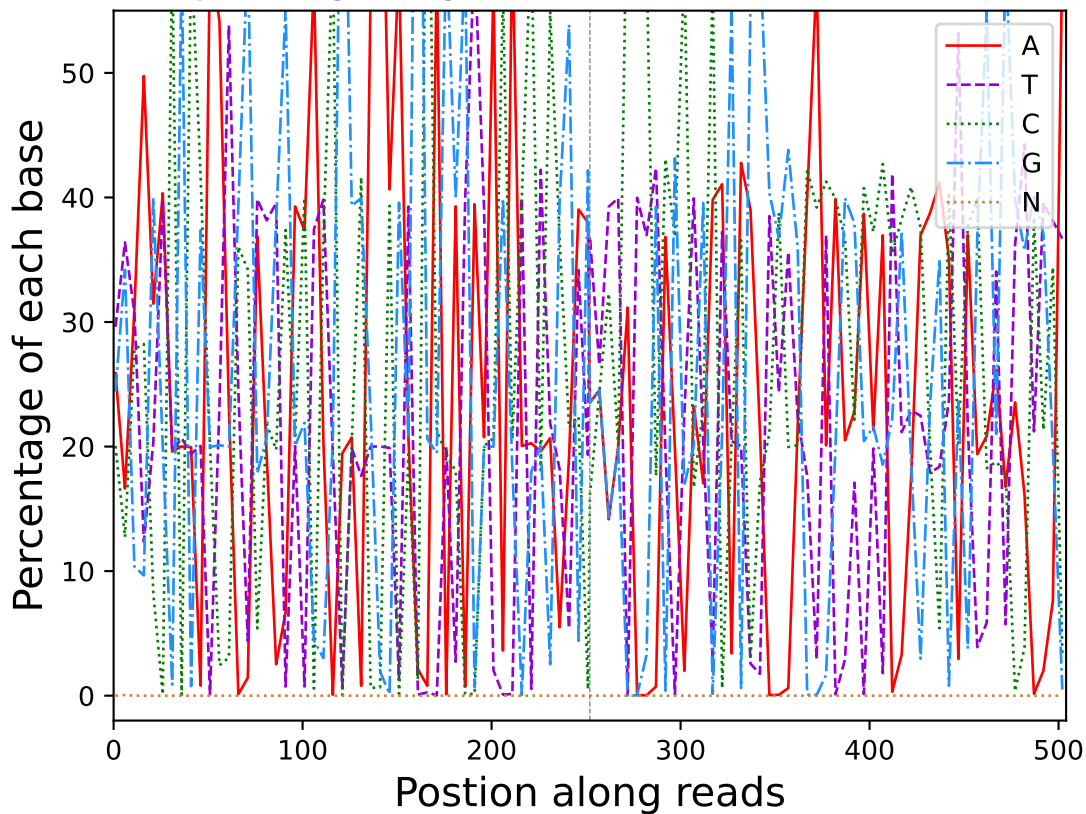
Base percentage along reads (R10221)
